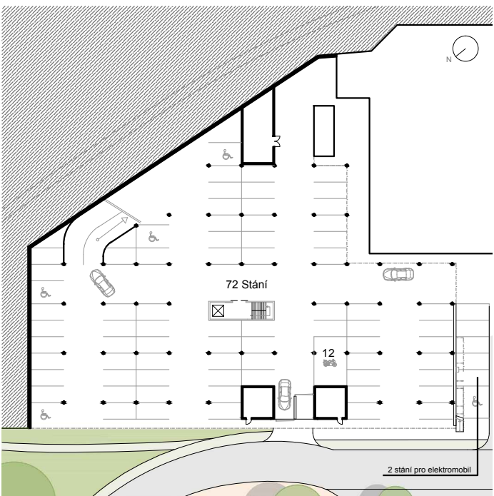
PARKING A 1 NP ± 0,00 m
