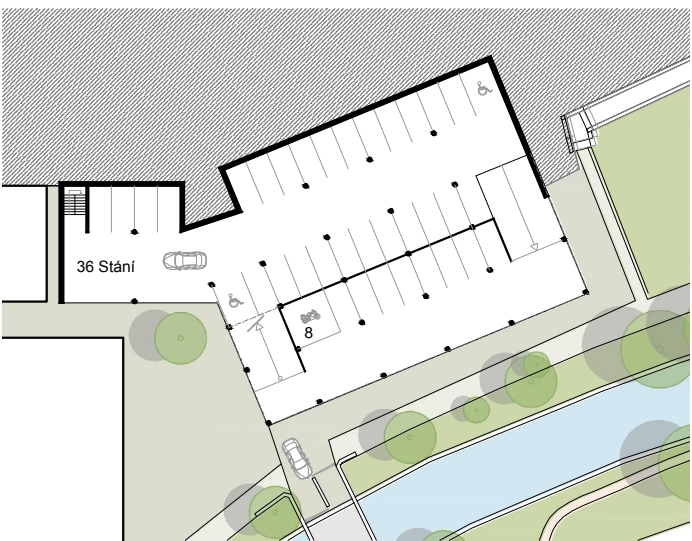
PARKING B 1 NP ± 0,00 m
