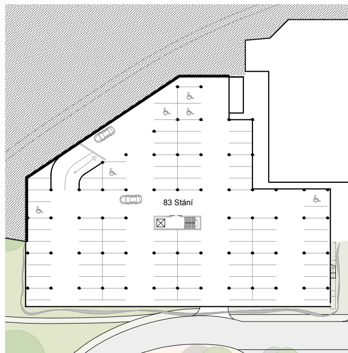
PARKING A 2 NP + 2,70 m
